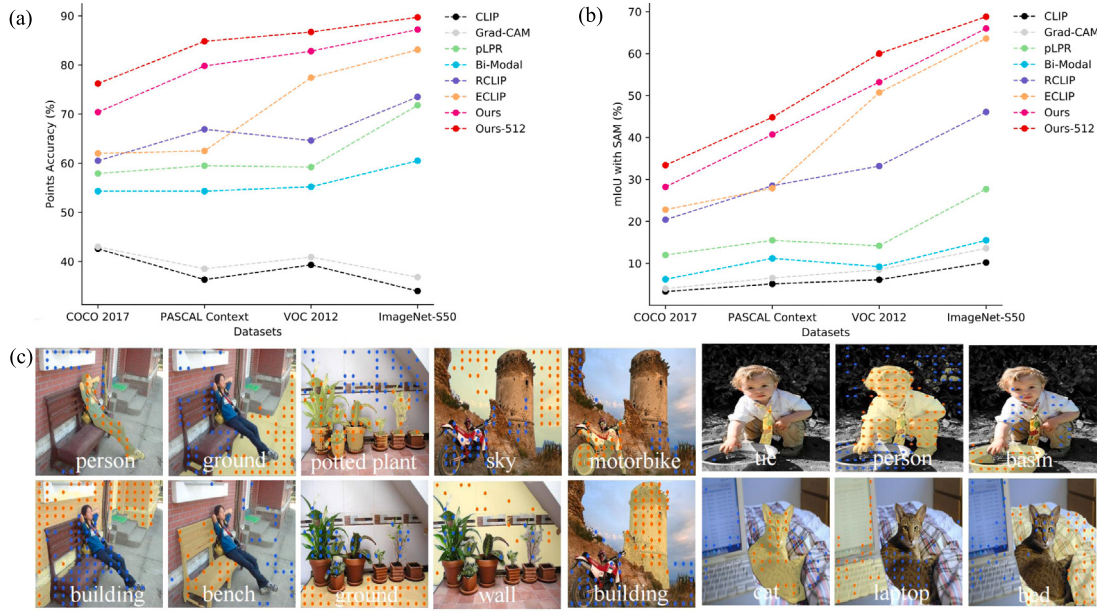
Fig. 10. Comparison of points accuracy (a) and mIoU (b) with SAM [30] among explainability methods on four datasets. Points and masks of our method are shown in (c). Note, all the input size is 224, except “Ours-512” at 512. (For interpretation of the references to color in this figure legend, the reader is referred to the web version of this article.)
