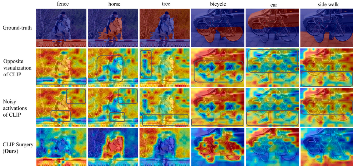
Fig. 1. The CAM of CLIP exhibits opposite and noisy visualizations, as indicated by the black boxes in the second and third rows, respectively. In contrast, our CLIP surgery addresses these issues, resulting in improved visualizations, as shown in the last row. The foregrounds are shown in red, while the backgrounds are indicated in blue. (For interpretation of the references to color in this figure legend, the reader is referred to the web version of this article.)
