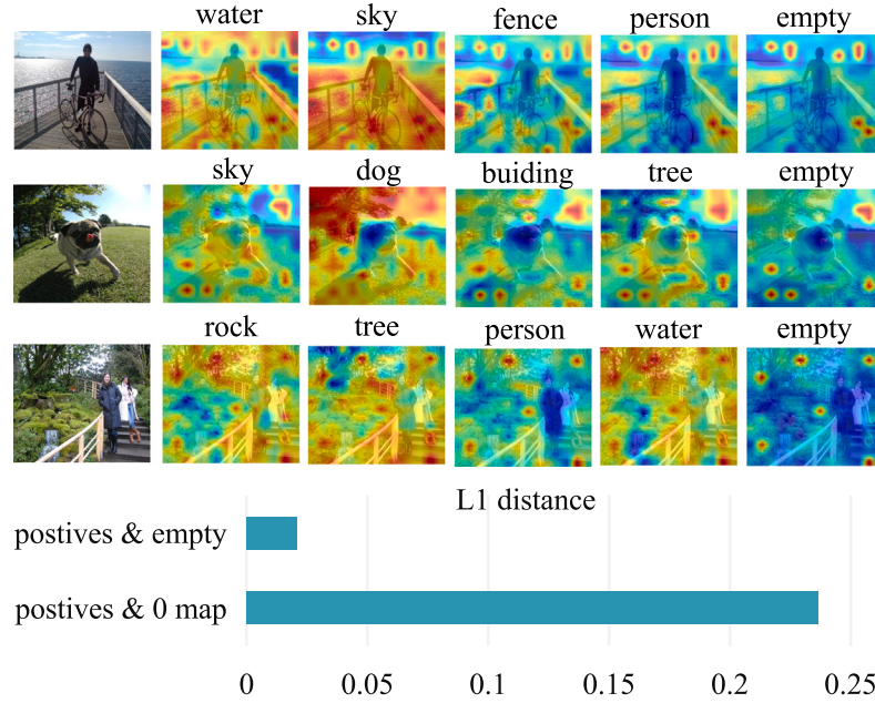
Fig. 6. Similarity maps from positive labels are similar to the map from an empty string, which produces redundant features irrelevant to any category. The bar chart indicates the overall L1 distance between positive maps vs. the empty map or the 0 map (no activation) on the PASCAL Context dataset [35], suggesting the predictions of CLIP among categories are highly related to redundant features.
