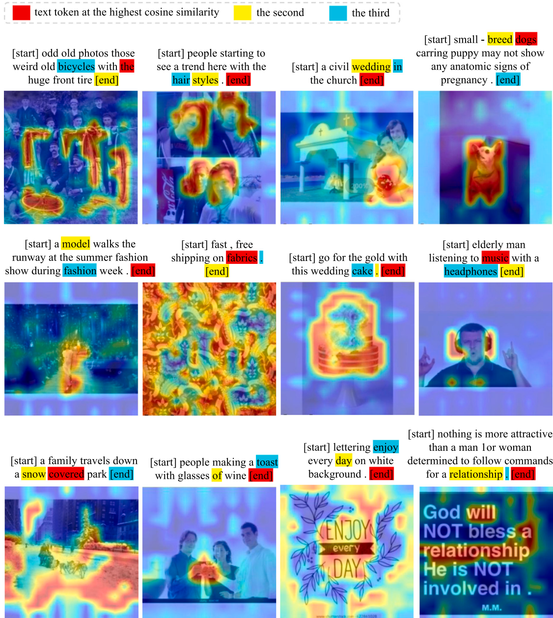
Fig. 11. Multimodal visualization to explain the image-text pairs used in the training process of CLIP. The visual explainability results are from the proposed CLIP Surgery, and textual explainability results are based on the cosine distance of each text token. [start] indicates the start text token and [end] means the end text token. Note that we mark the text token at the highest cosine similarity in red, then draw the second in yellow and blue for the third. (For interpretation of the references to color in this figure legend, the reader is referred to the web version of this article.)
