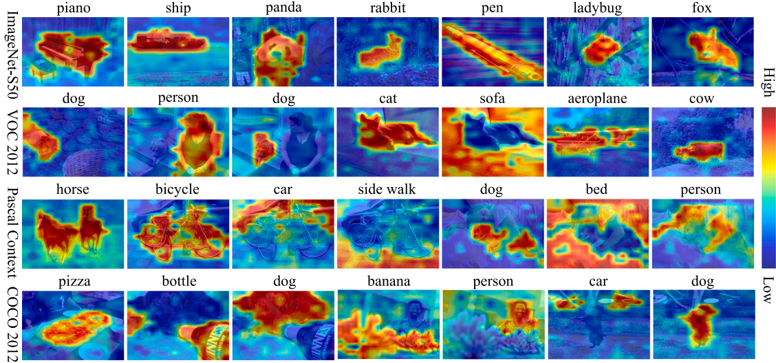
Fig. 8. Our CLIP Surgery solves the explainability problems and provides good visualizations on varied datasets.
