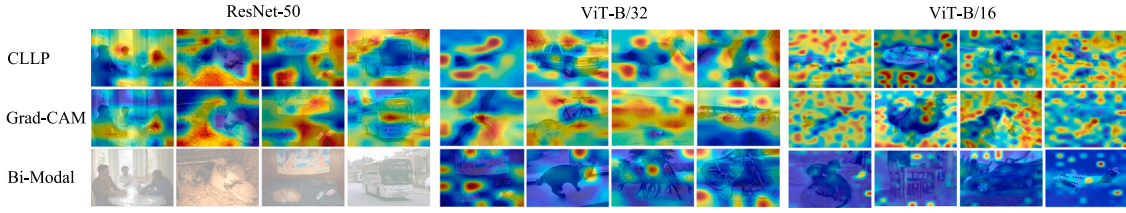
Fig. 3. CLIP shows opposite visualization with noisy activations, which are common on varied backbones (ResNet [34], ViT [21]) and methods (Grad-CAM [3], Bi-modal [15]). Note, Bi-modal for ViT is not applicable to ResNet.
