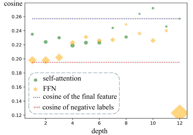
Fig. 5. Analysis for intermediate self-attention blocks (green) and feed-forward networks (FFNs, colored in yellow) at different depths via the affinity in Eq. (5). The blue line indicates the mean cosine of all positive labels on the VOC 2012 dataset [19] using backbone ViT-B/16, and the red line is that of negative labels. All scatters are the mean cosine of positive labels and are expected to be close to the blue line. Larger scatters indicate the features of this block are more inconsistent with the final prediction. (For interpretation of the references to color in this figure legend, the reader is referred to the web version of this article.)
