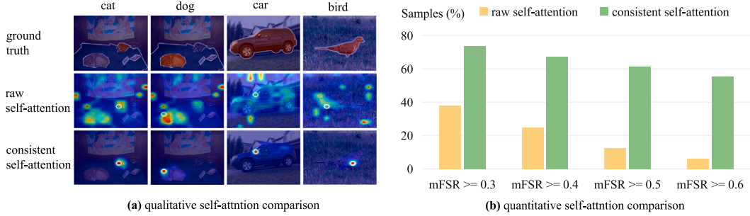
Fig. 4. The raw self-attention pays more attention to backgrounds, while the proposed consistent self-attention corrects it. (a) Qualitative comparison between the raw self-attention and our consistent self-attention at the token of the highest score on the last layer. The raw self-attention pays much attention to the opposite semantic regions, while our consistent self-attention links nearby tokens at the same semantics. (b) The quantitative comparison for self-attention focuses on foregrounds. Note, the y-axis indicates the sample ratio whose mFSR is higher than a threshold, and mFSR measures the attention degree on the foregrounds as Eq. (4).
