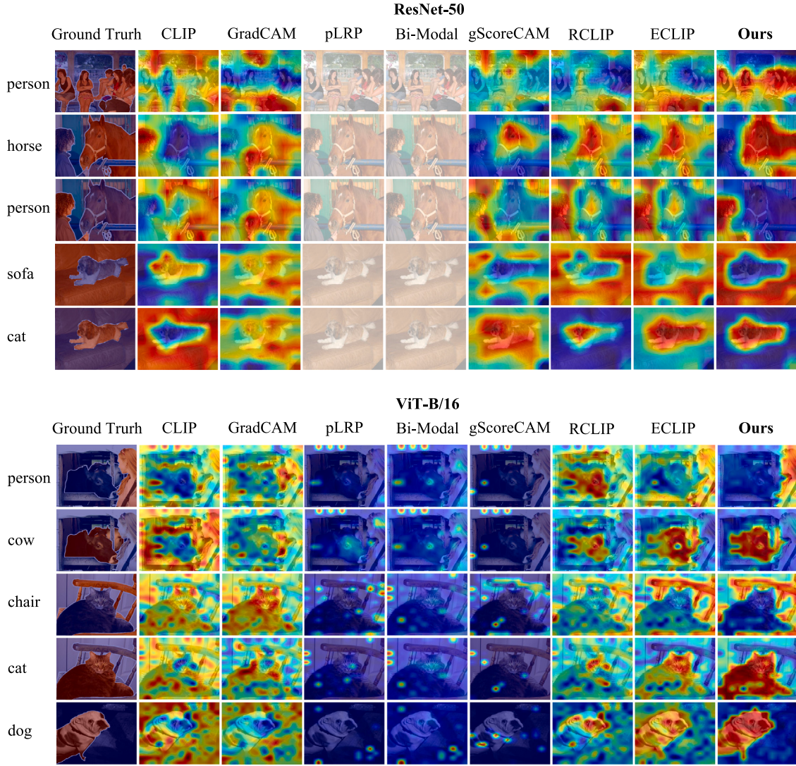
Fig. 9. Visual comparison between our CLIP Surgery with state-of-the-art explainability methods on VOC 2012 [19]. Note the foregrounds are colored in red, and the white mask indicates this method is not applicable to this backbone. Our visualization quality is much better than other methods for both ResNet and ViT, without any fine-tuning like ECLIP [11] or back-propagation in GradCAM [3]. Besides, our method is not limited by certain backbones such as pLRP [18], Bi-Modal [15], and gScoreCAM [16]. (For interpretation of the references to color in this figure legend, the reader is referred to the web version of this article.)
