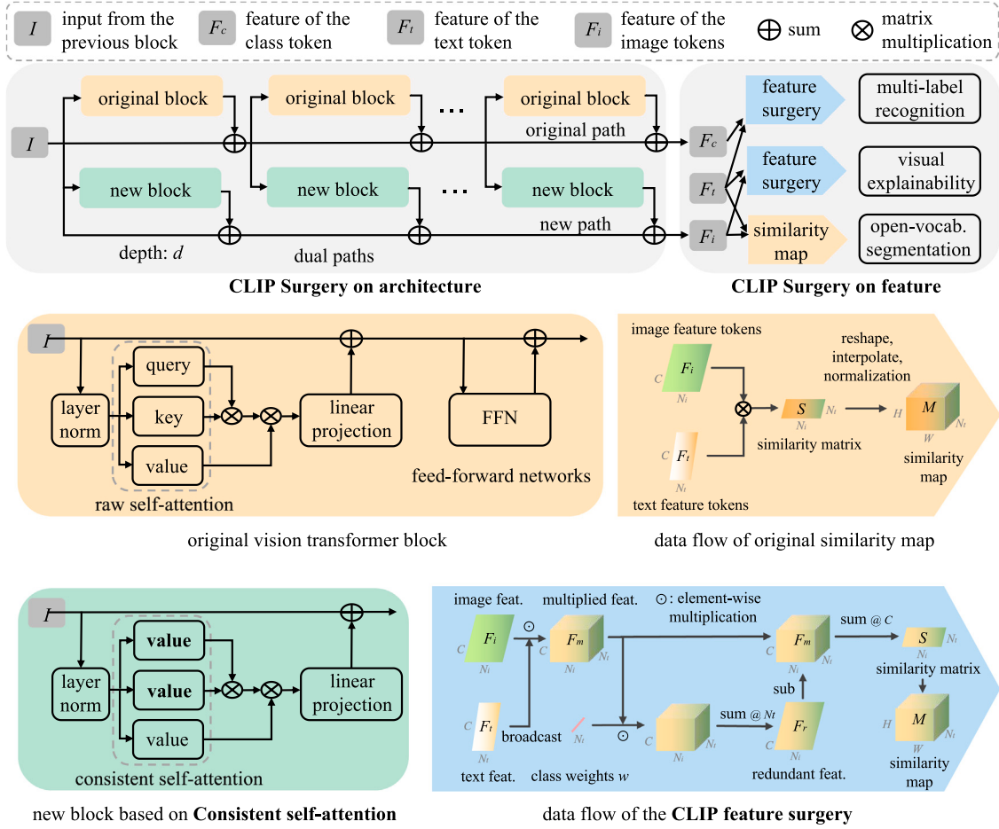
Fig. 2. Data flow of the proposed method and comparison with the original architecture. The top part indicates the overall framework of clip surgery, including a dual paths structure to introduce new blocks with feature surgery in the last. The original modules are colored in yellow at the middle part. In comparison, the new block is based on the consistent self-attention using homogeneous parameters without feed-forward networks (FFN). The data flow of feature surgery is given in the right bottom part to mitigate redundant features across texts. (For interpretation of the references to color in this figure legend, the reader is referred to the web version of this article.)
